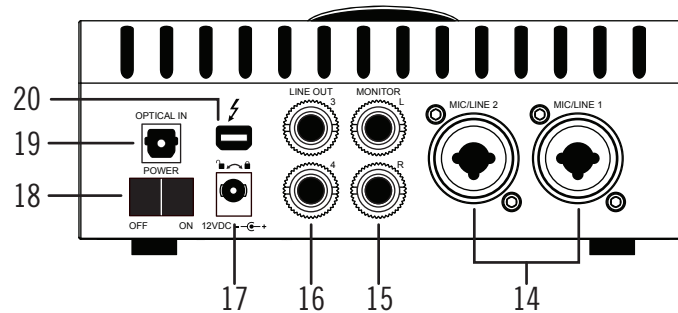
Apollo Twin's rear panel elements
