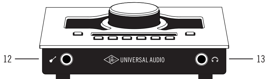
Apollo Twin's front panel elements
