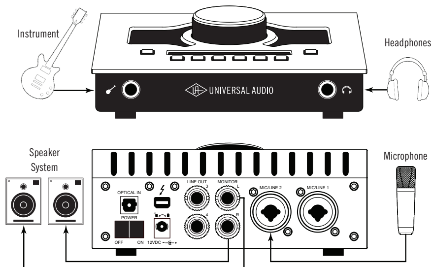
Typical setup connections
